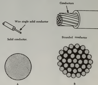
FIGURE 4-80. Two types of aircraft wire.
